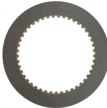
Gradall Clutch Plate - Friction 0420-0341
