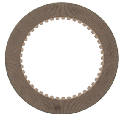
Galion Clutch Plate - Friction 72330
