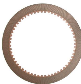
Grove Crane Clutch Plate - Friction 9904101483
