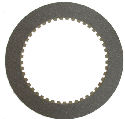
Borg Warner Clutch Plate - Friction 1021-666-002
