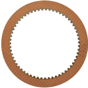
Borg Warner Clutch Plate - Friction 1017-666-001
